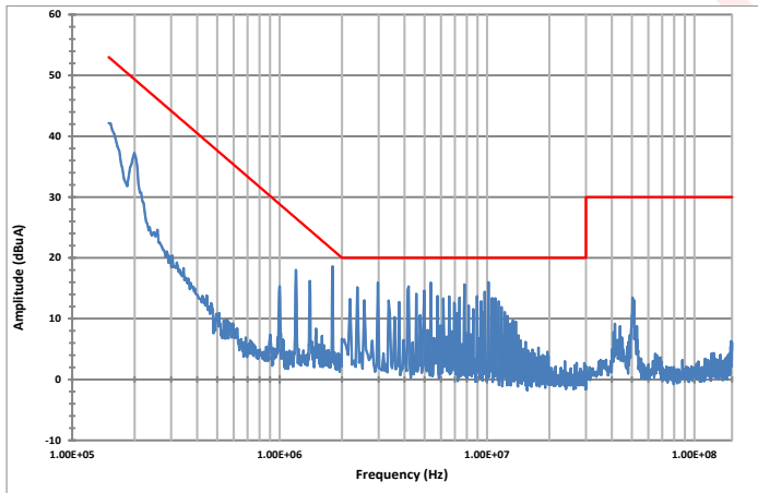
Figure 21: D0-160G conducted emissions of ACF-U-230-HT filter and APFIC-U converter at full load, 115Vrms 400 Hz, category M limit.
